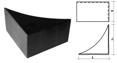
PROTEGGIANGOLO 100X100X60
